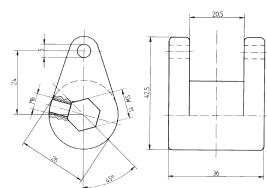
For sekskant stål SW11 [DIN 176]
